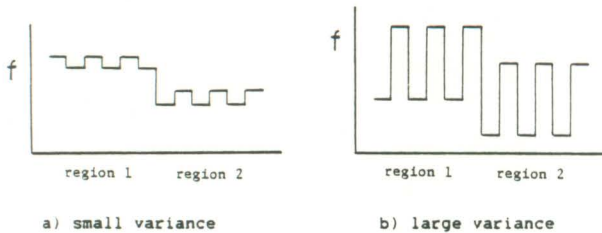
Figure 6 : Examples of regions with the same criterion values but different variances.
